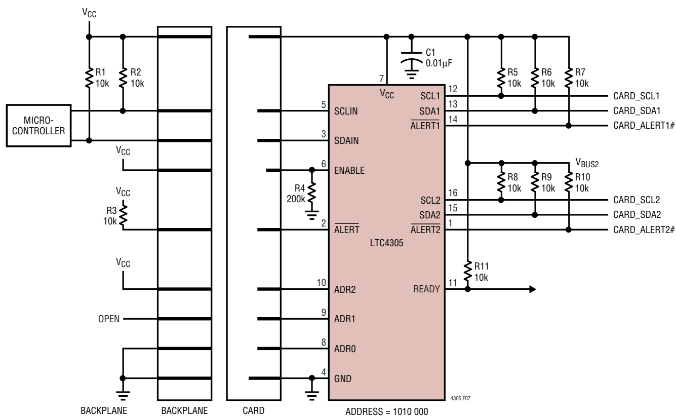
Figure 7. Hot-Swapping Application
