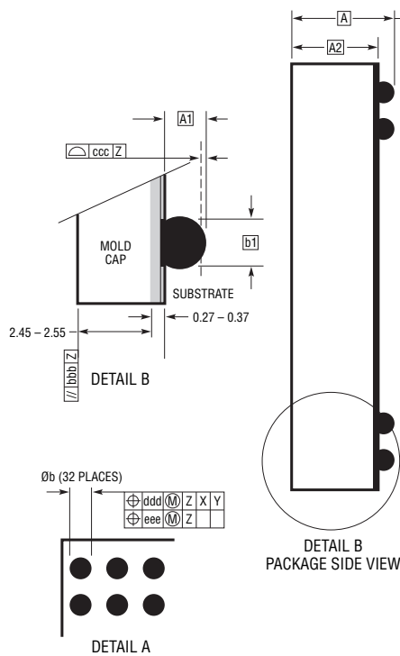
DETAIL A
