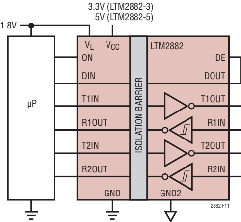
Figure 11. 1.8V Microprocessor Interface
