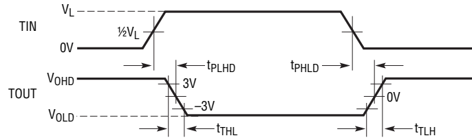
Figure 1. Driver Slew Rate and Timing Measurement
