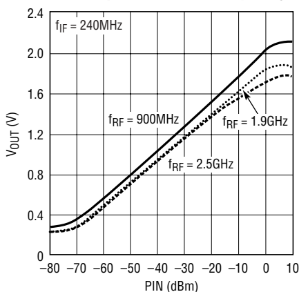
Output Voltage vs RF Input Power and Frequency
