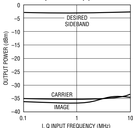
Baseband Frequency Response I/Q Amplitude = 1\text{V}_{P-P}
