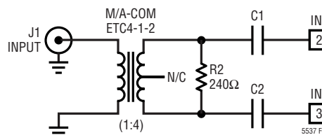
Figure 5. Differential Input Matching to 200 \Omega
