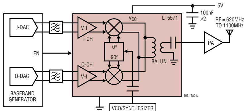
Direct Conversion Transmitter Application
