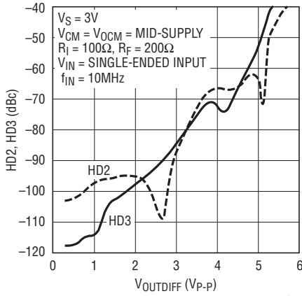
Distortion vs Output Amplitude
