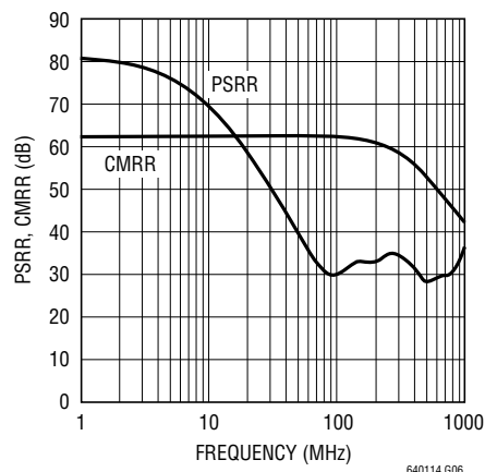
PSRR and CMRR vs Frequency
