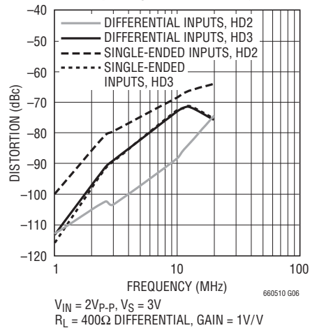
Harmonic Distortion vs Frequency, BIAS Floating
