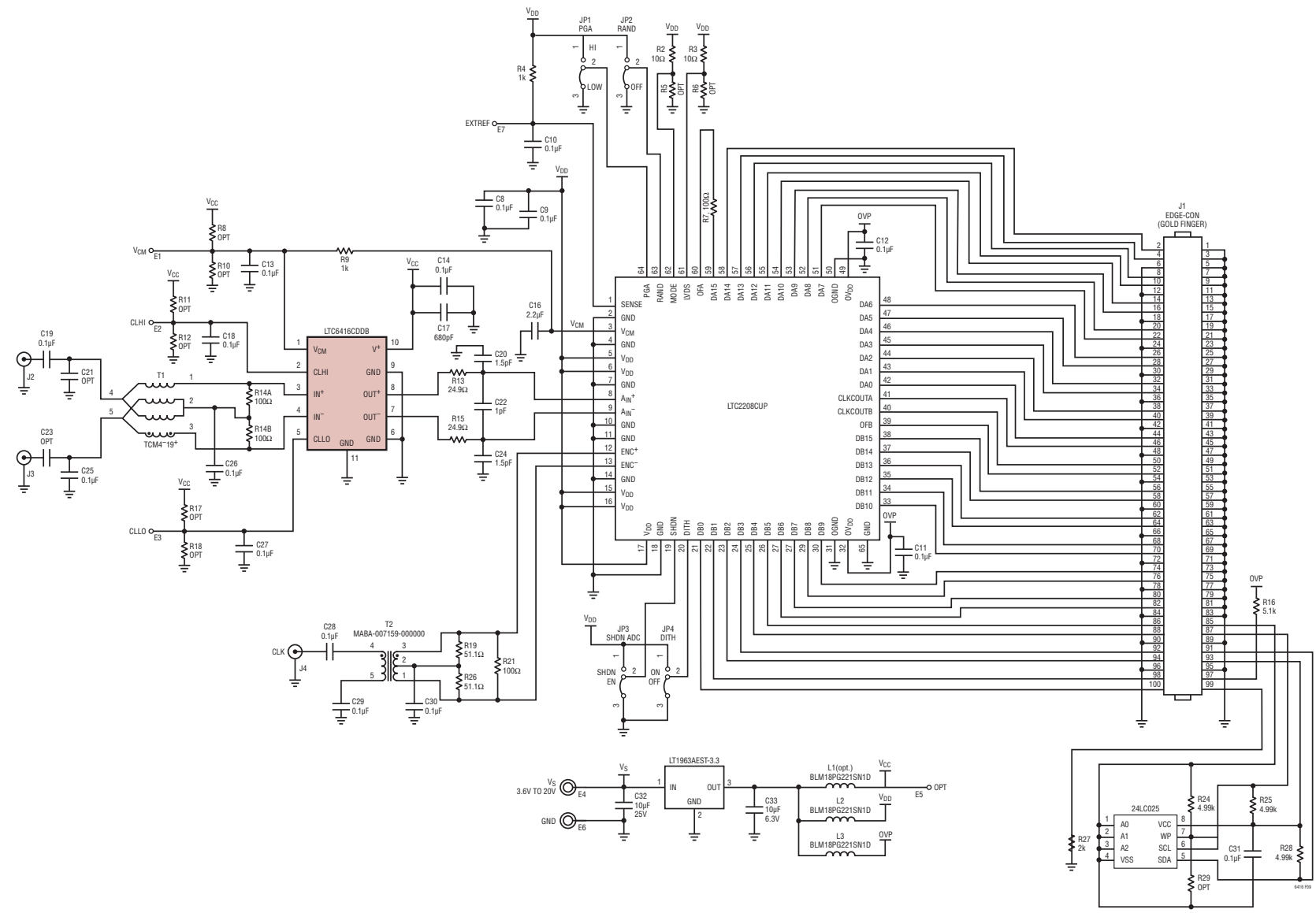
Figure 9. Demo Board DC1257B Schematic (Test Circuit B)
