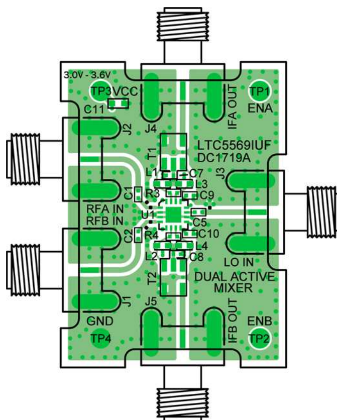
Figure 2. Evaluation Board Layout
