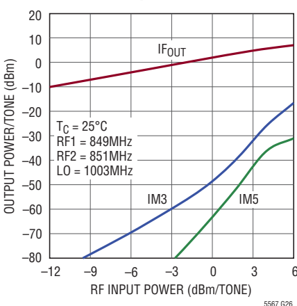
2-Tone IF Output Power, IM3 and IM5 vs RF Input Power
