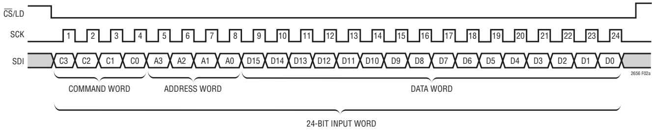
Figure 2a. LTC2656-16 24-Bit Load Sequence (Minimum Input Word) LTC2656-12 SDI Data Word: 12-Bit Input Code + 4 Don't-Care Bits
