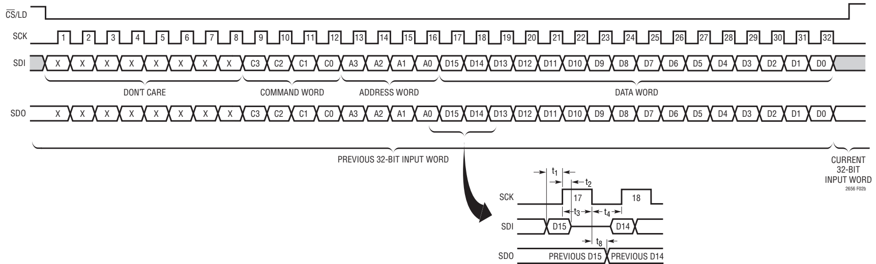
Figure 2b. LTC2656-16 32-Bit Load Sequence LTC2656-12 SDI/SDO Data Word: 12-Bit Input Code + 4 Don't-Care Bits
