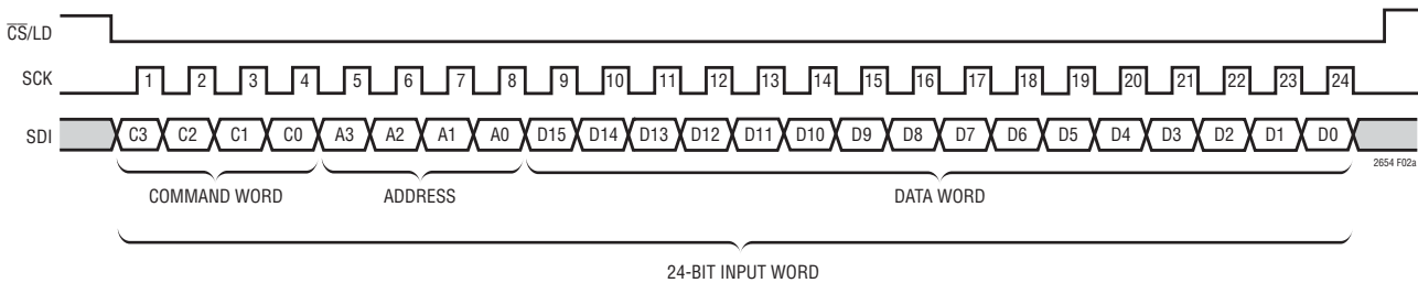
Figure 2a. LTC2654-16 24-Bit Load Sequence (Minimum Input Word) LTC2654-12 SDI Data Word: 12-Bit Input Code + 4 Don't Care Bits
