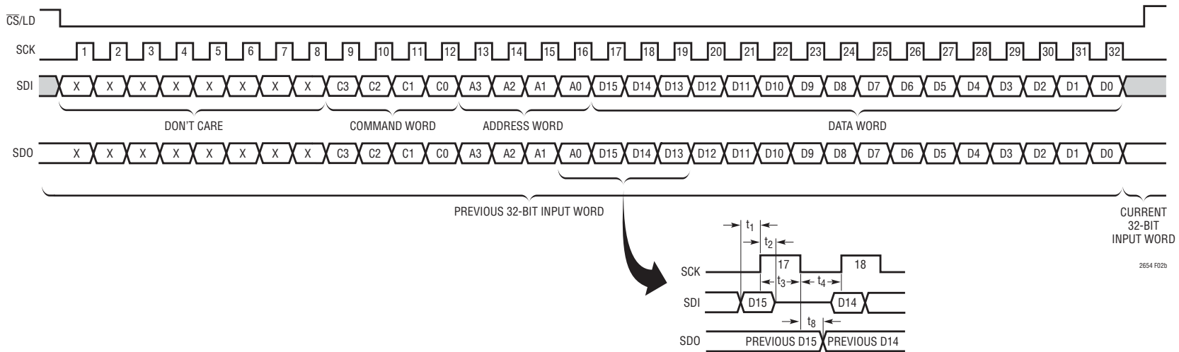
Figure 2b. LTC2654-16 32-Bit Load Sequence. LTC2654-12 SDI/SDO Data Word: 12-Bit Input Code + 4 Don't Care Bits
