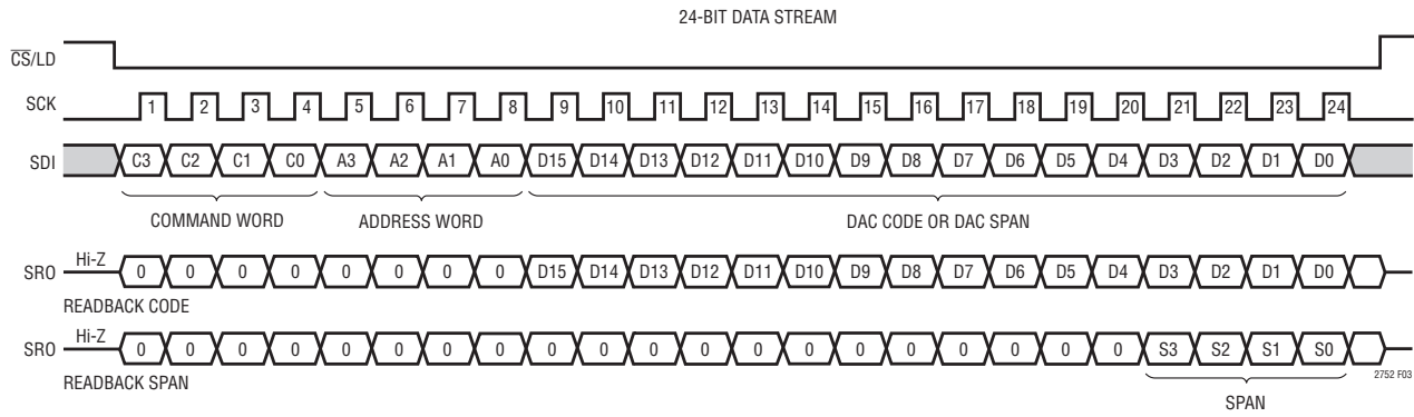
Figure 3a. 24-Bit Instruction Sequence
