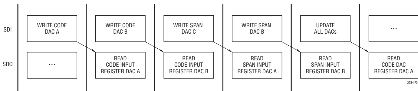
Figure 4. Rolling Readback
