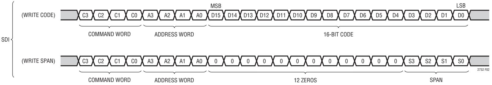
Figure 2. Serial Input Write Sequence
