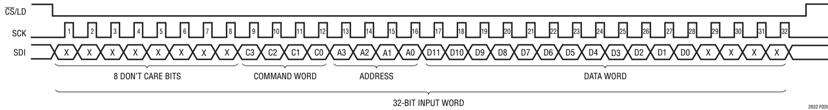
Figure 3b. LTC2632-12 32-Bit Load Sequence LTC2632-10 SDI Data Word: 10-Bit Input Code + 6 Don't-Care Bits; LTC2632-8 SDI Data Word: 8-Bit Input Code + 8 Don't-Care Bits
