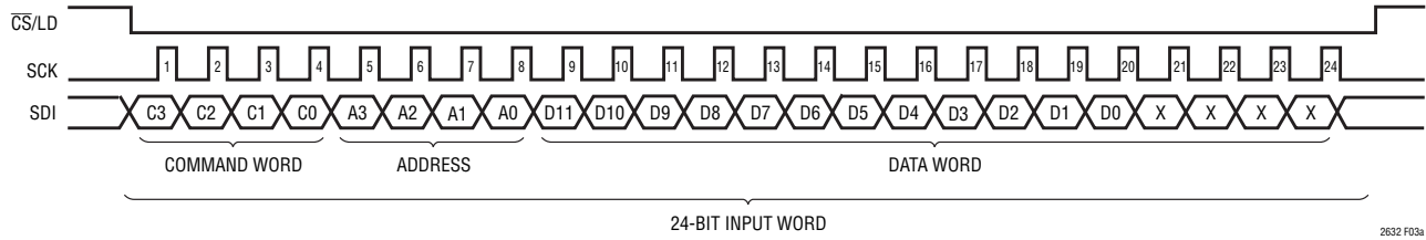
Figure 3a. LTC2632-12 24-Bit Load Sequence (Minimum Input Word) LTC2632-10 SDI Data Word: 10-Bit Input Code + 6 Don't-Care Bits; LTC2632-8 SDI Data Word: 8-Bit Input Code + 8 Don't-Care Bits
