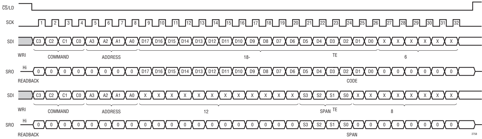
Figure 2. Serial Input and Output Sequences
