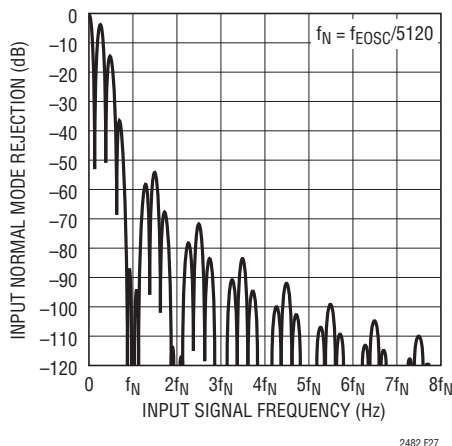
Figure 27. Input Normal Mode Rejection at DC
