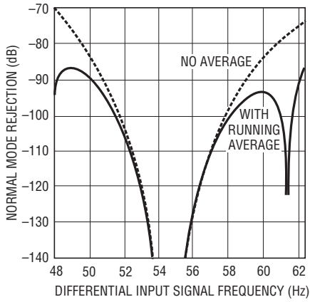
Figure 29. Input Normal Mode Rejection 2x Speed Mode with and Without Running Averaging
