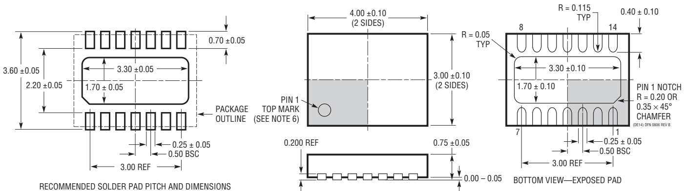
DE Package 14-Lead Plastic DFN (4mm × 3mm) (Reference LTC DWG # 05-08-1708 Rev B)
