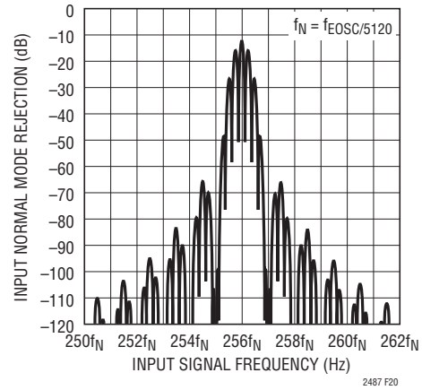
Figure 20. Input Normal Mode Rejection at f_s = 256 \cdot f_N
