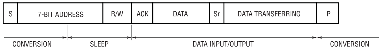
Figure 6. Conversion Sequence
