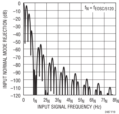
Figure 19. Input Normal Mode Rejection at DC
