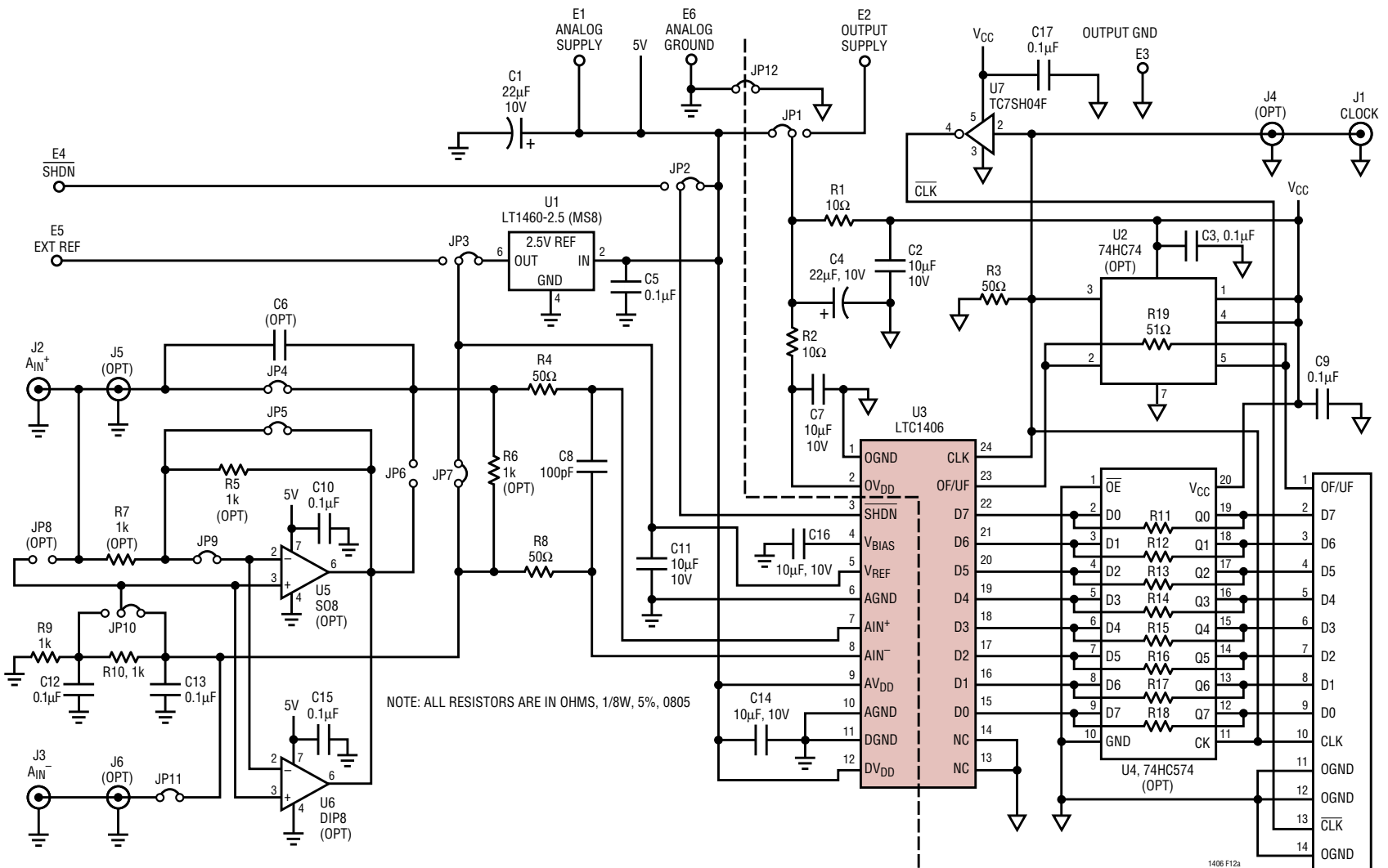
Figure 12a. Suggested Evaluation Circuit Schematic
