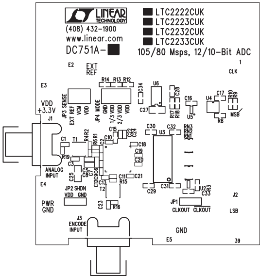
Silkscreen Top
