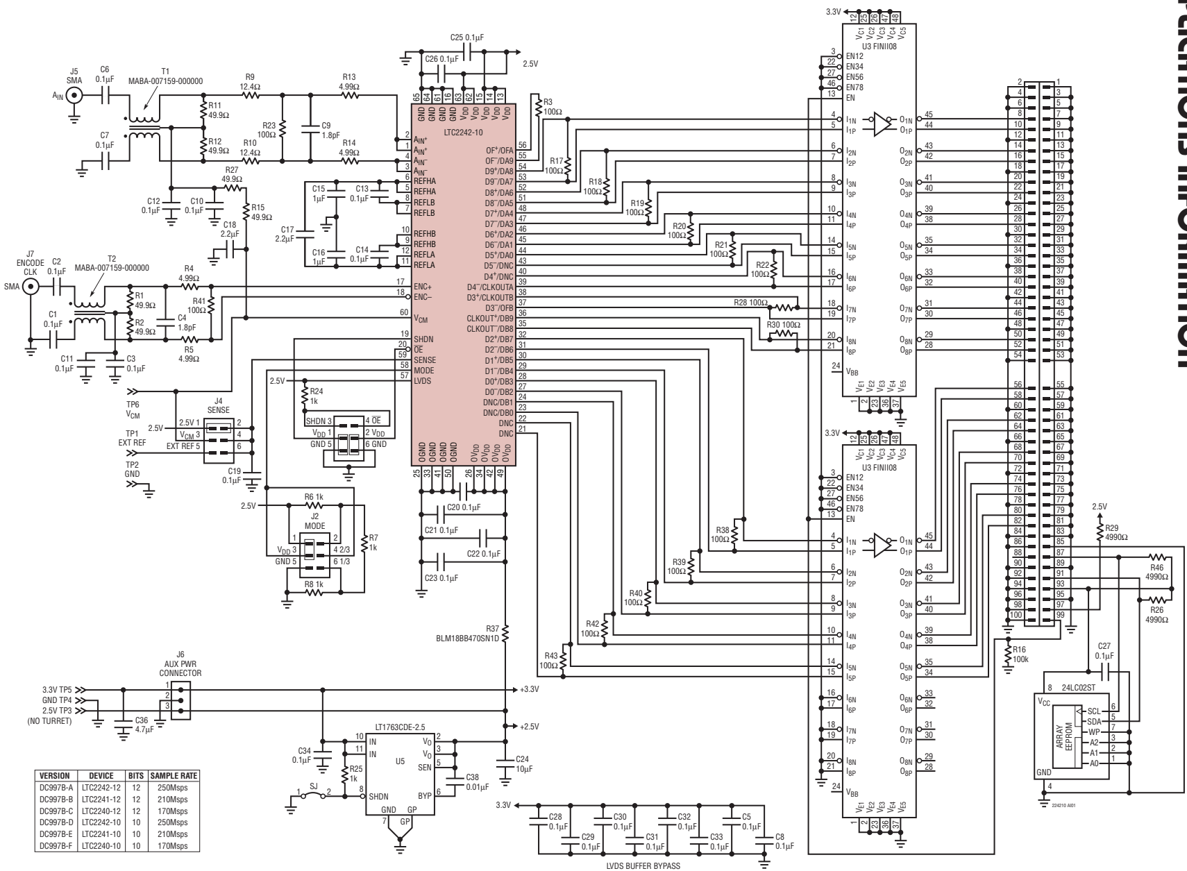
Evaluation Circuit Schematic of the LTC2242-10
