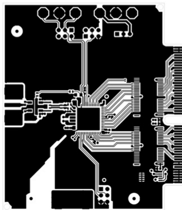
Layer 1 Component Side
