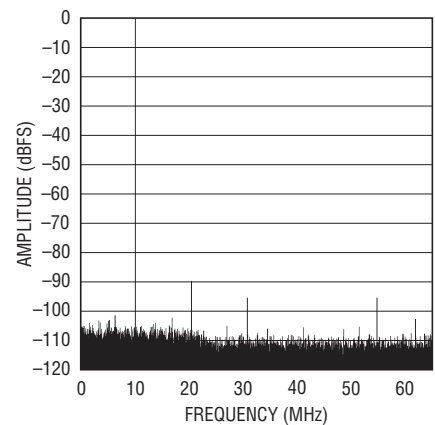
32k Point FFT, f_{IN} = 140.11\text{MHz} , -1dBFS, PGA = 1, RAND = "On", Dither "Off"
