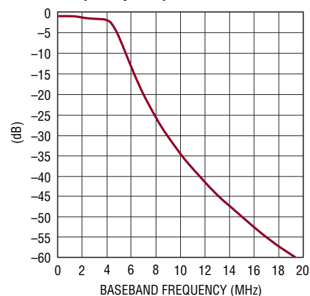
LTM9004-AA, Baseband Frequency Response
