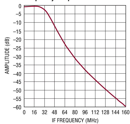
LTM9004-AD, Baseband Frequency Response
