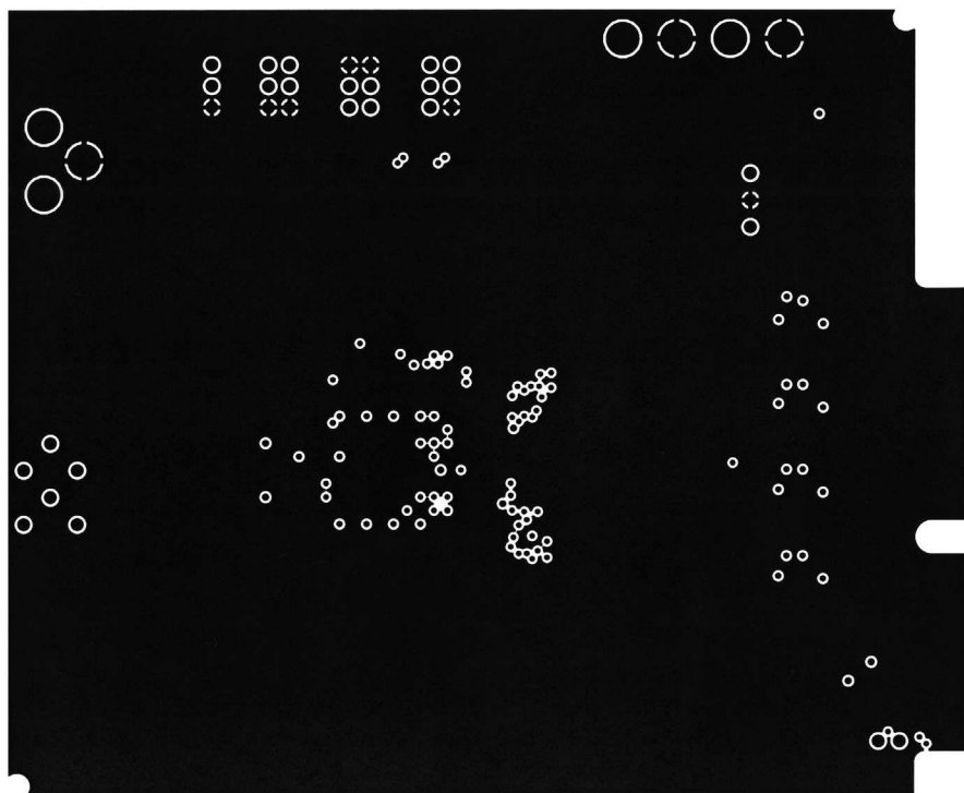
Figure 13. Layer 3
