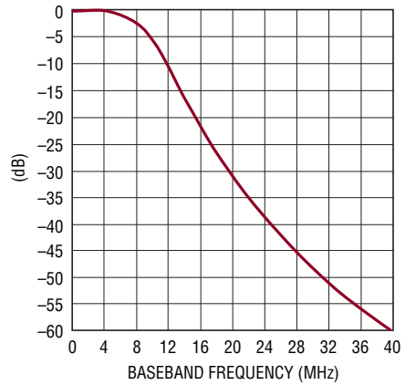
LTM9004-AB, Baseband Frequency Response
