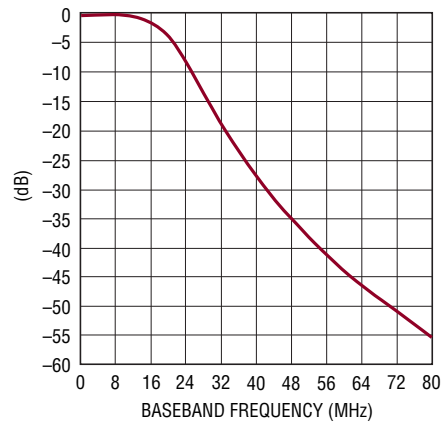
LTM9004-AC, Baseband Frequency Response
