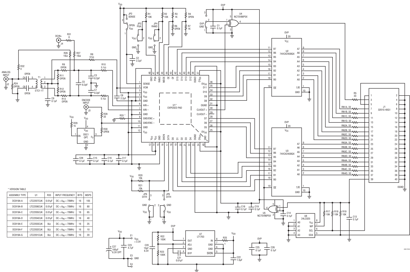
Evaluation Circuit Schematic of the LTC2201
