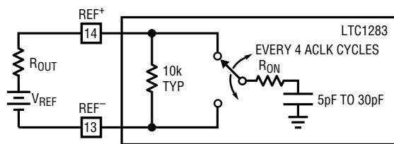
Figure 14. Reference Input Equivalent Circuit
