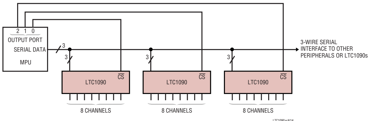
Figure 5. Several LTC1090's Sharing One 3-Wire Serial Interface
