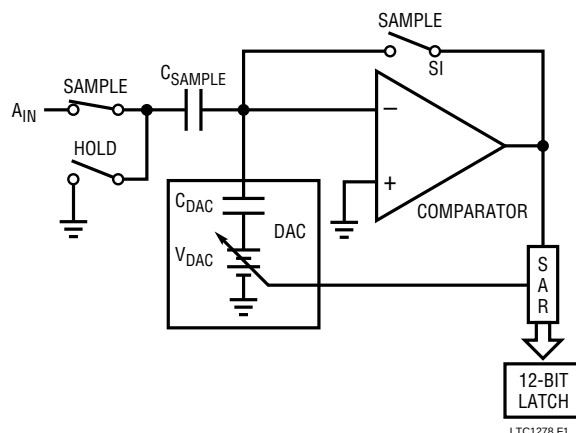
Figure 1. A_{IN} Input
