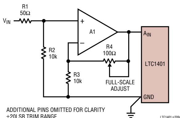
Figure 9a. LTC1401 Full-Scale Adjust Circuit
