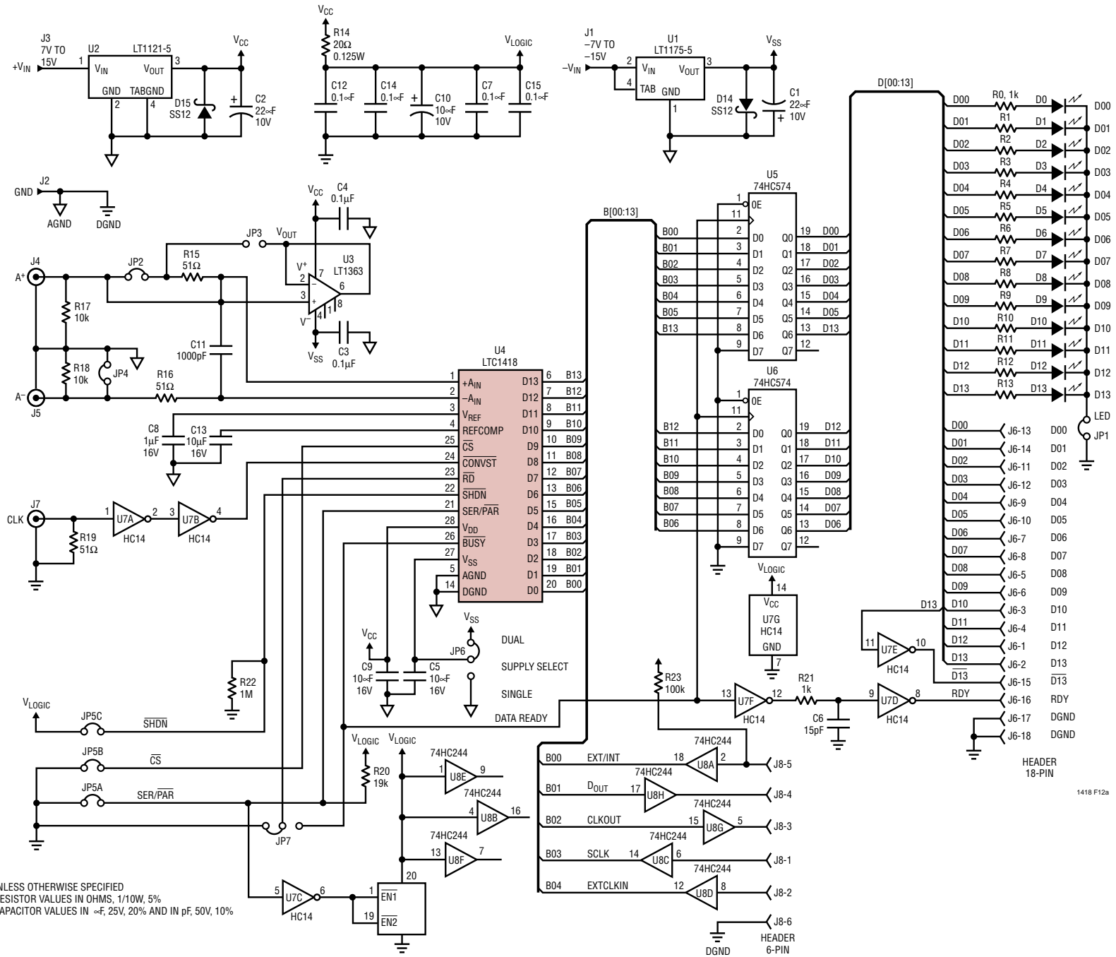
Figure 12a. Suggested Evaluation Circuit Schematic
