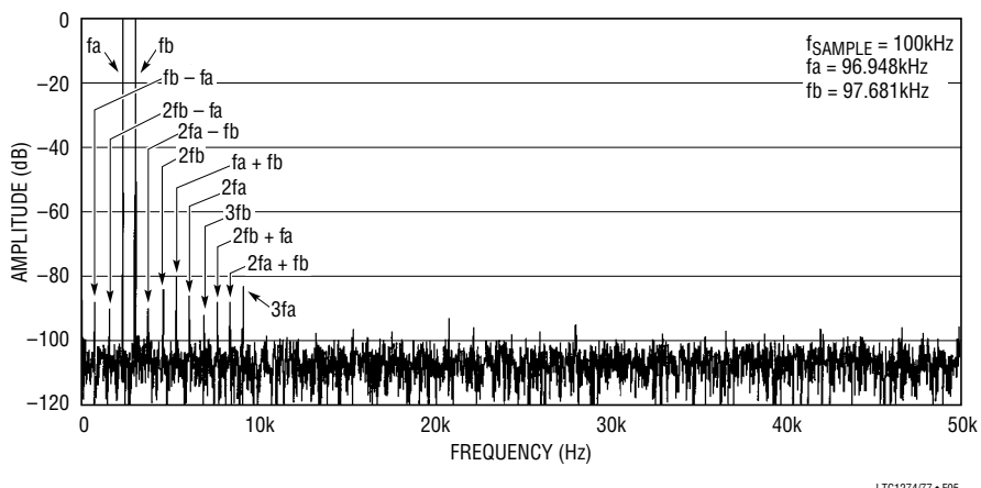
Figure 5. Intermodulation Distortion
