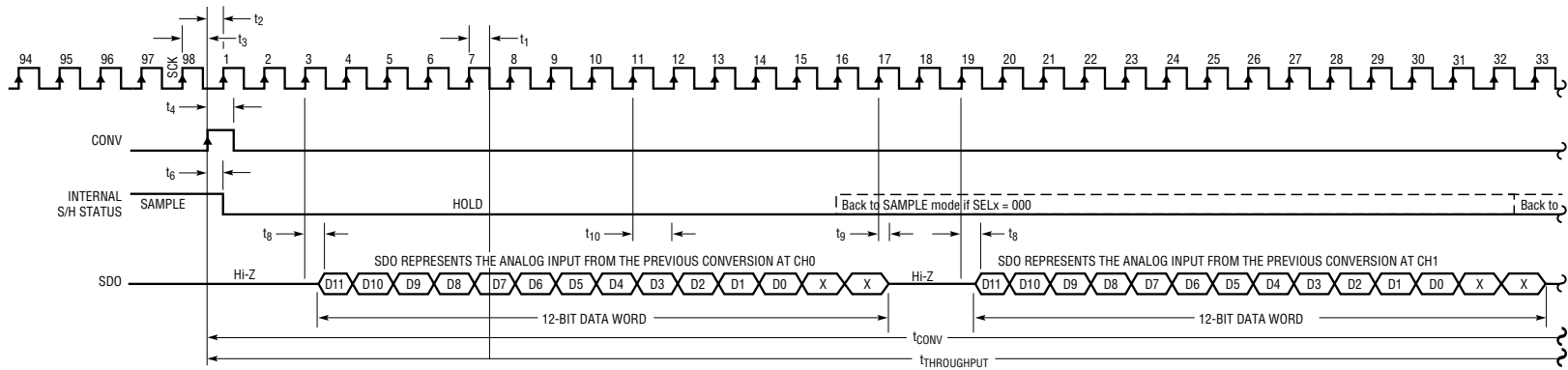
LTC1408-12 Timing Diagram
