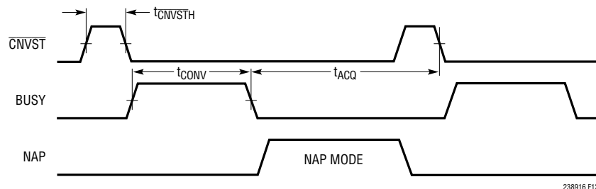
Figure 12. Nap Mode Timing for the LTC2389-16
