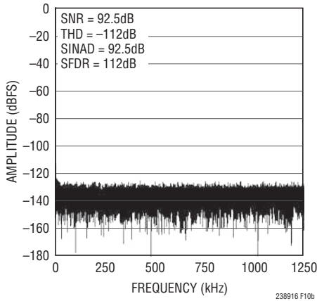
Figure 10b. 32k Point FFT f_{\text{SMPL}} = 2.5\text{Msps} , f_{\text{IN}} = 2\text{kHz} , for Circuit Shown in Figure 10a; Driven with Unipolar Inputs
