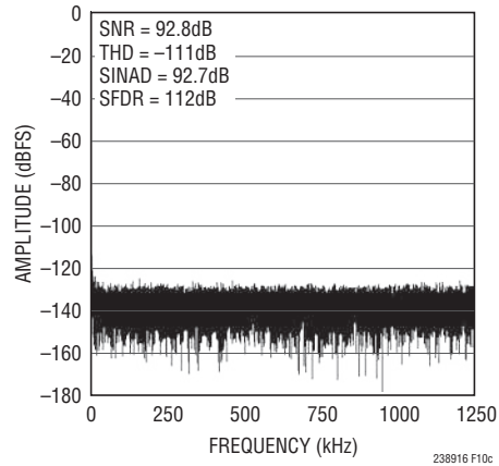
Figure 10c. 32k Point FFT f_{\text{SMPL}} = 2.5\text{Msps} , f_{\text{IN}} = 2\text{kHz} , for Circuit Shown in Figure 10a; Driven with Bipolar Inputs
