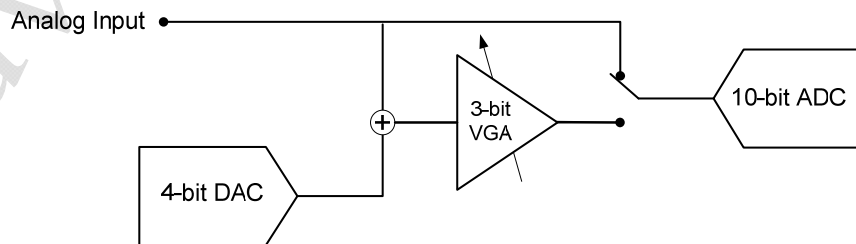
Figure 13 Analog to Digital Chain
