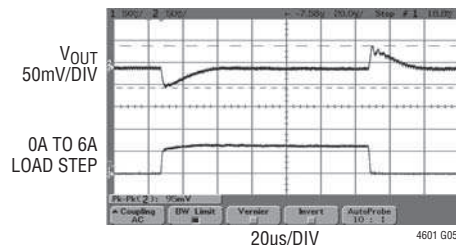
1.5V Transient Response
