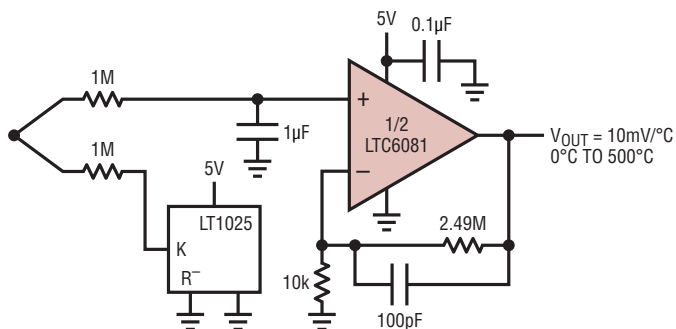
Thermocouple Amplifier
