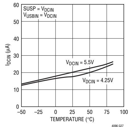
Shutdown Supply Current vs Temperature and V_DCIN
