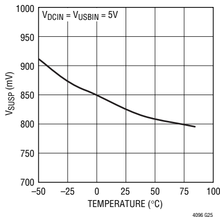
SUSP Pin Threshold Voltage (On-to-Off) vs Temperature
