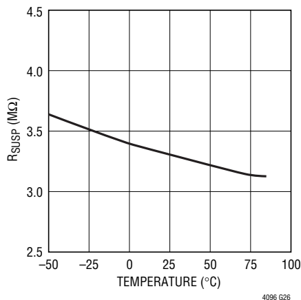
SUSP Pin Pulldown Resistance vs Temperature
