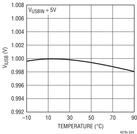
IUSB Pin Voltage vs Temperature (Constant-Current Mode)
