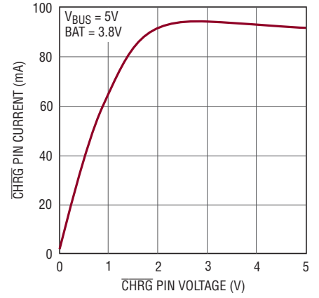
CHRG Pin Current vs Voltage (Pull-Down State)
