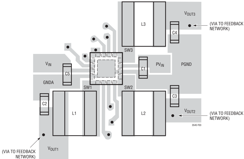
Figure 3. Layout Diagram
