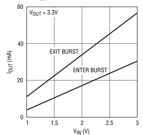
Burst Mode Threshold Current vs V IN
