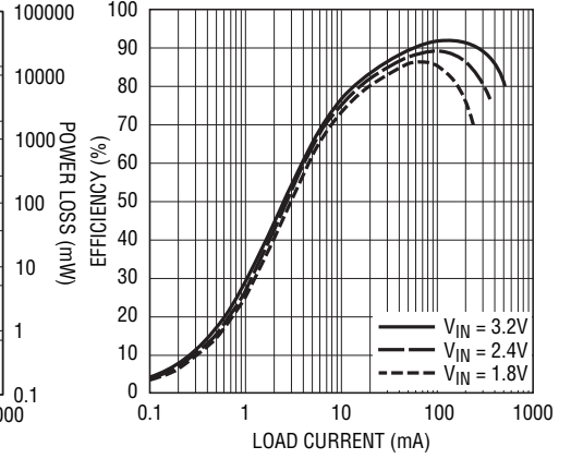
2-Cell to 5V Efficiency vs Load Current (LTC3499B Only)
