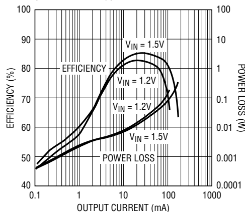
Single-Cell to 3.3V Efficiency (LTC3429 Only)
