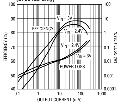
2-Cell to 5V Efficiency (LTC3429 Only)
