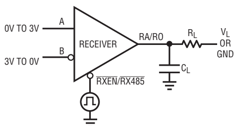
Figure 7. RS485 Receiver Enable and Disable Timing Measurements (Note 5)
