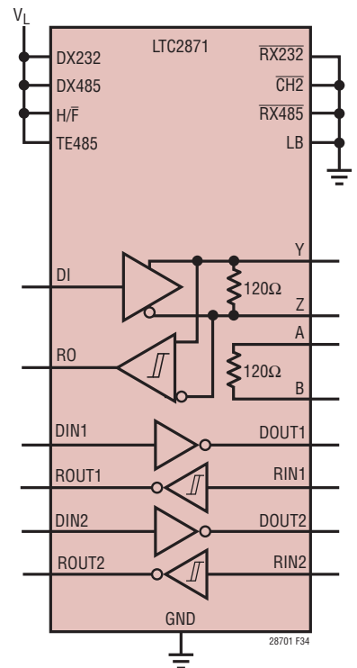
Figure 34. LTC2871 in RS485 and RS232 Mode, RS485 Half-Duplex, Terminated
