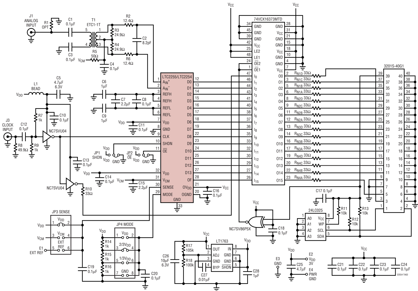
Evaluation Circuit Schematic of the LTC2255/LTC2254
