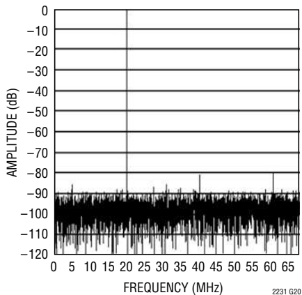
LTC2231: 8192 Point FFT, f_{IN} = 250\text{MHz} , -1\text{dB} , 2\text{V} Range
