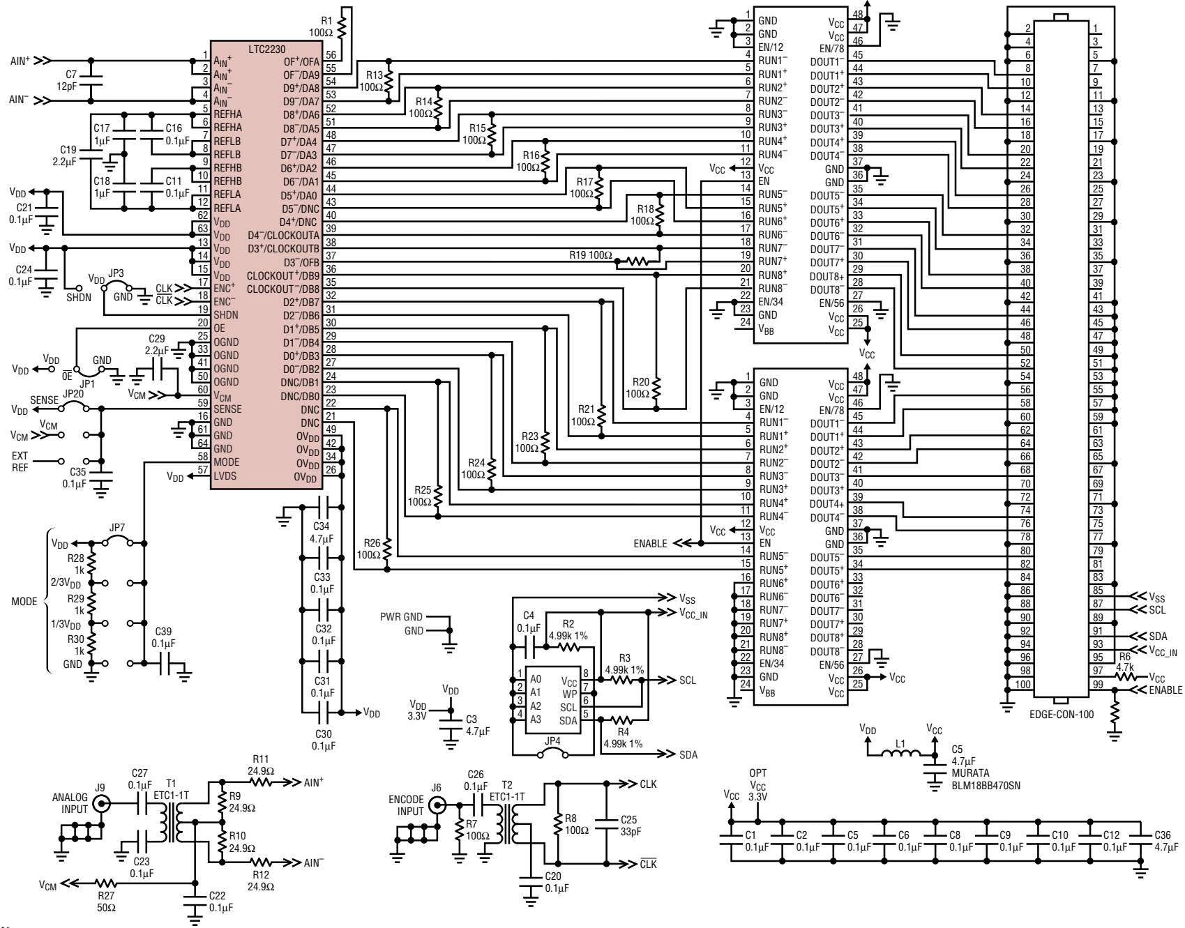
Evaluation Circuit Schematic of the LTC2230
