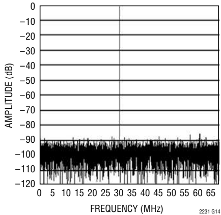
LTC2231: 8192 Point FFT, f_{IN} = 30\text{MHz} , -1\text{dB} , 2\text{V} Range
