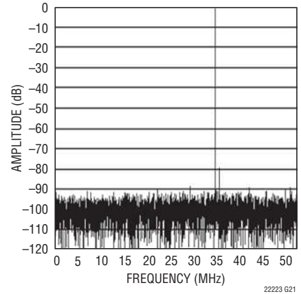
LTC2222: 8192 Point FFT, f_{IN} = 140\text{MHz} , -1\text{dB} , 1\text{V} Range
