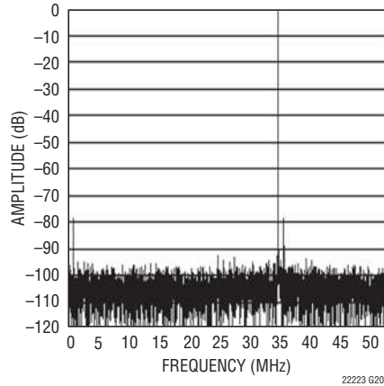
LTC2222: 8192 Point FFT, f_{IN} = 140\text{MHz} , -1\text{dB} , 2\text{V} Range
