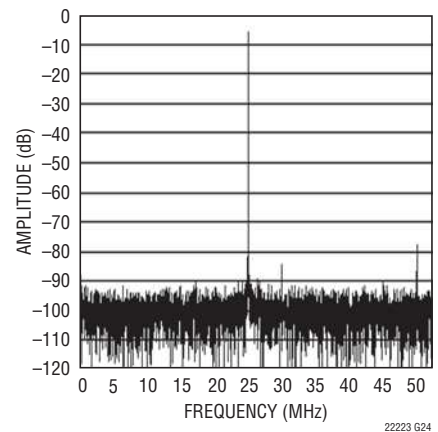
LTC2222: 8192 Point FFT, f_{IN} = 500\text{MHz} , -6\text{dB} , 1\text{V} Range
