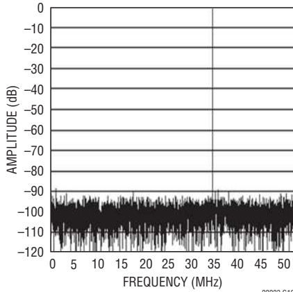
LTC2222: 8192 Point FFT, f_{IN} = 70\text{MHz} , -1\text{dB} , 1\text{V} Range
