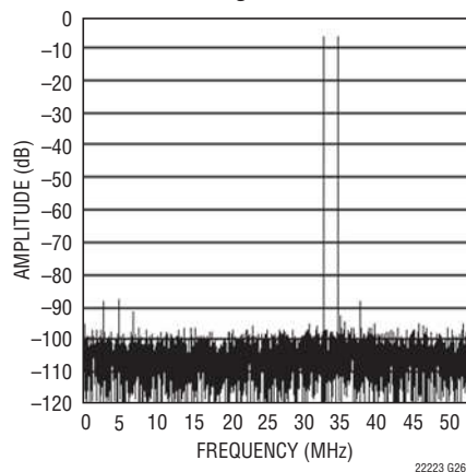
LTC2222: 8192 Point 2-Tone FFT, f_{IN} = 138\text{MHz} and 140\text{MHz} , -7\text{dB} Each, 1\text{V} Range
