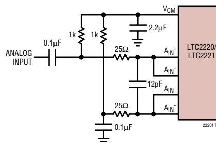
Figure 5. Single-Ended Drive
